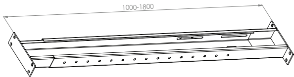
Telescopic Beam
