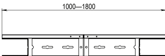
Telescopic Beam
